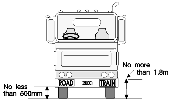
Positioning of a warning sign
